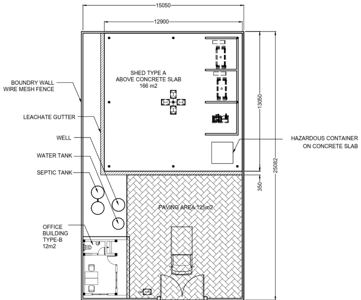
Figure 5: ISWMC concept of Thinadhoo island
