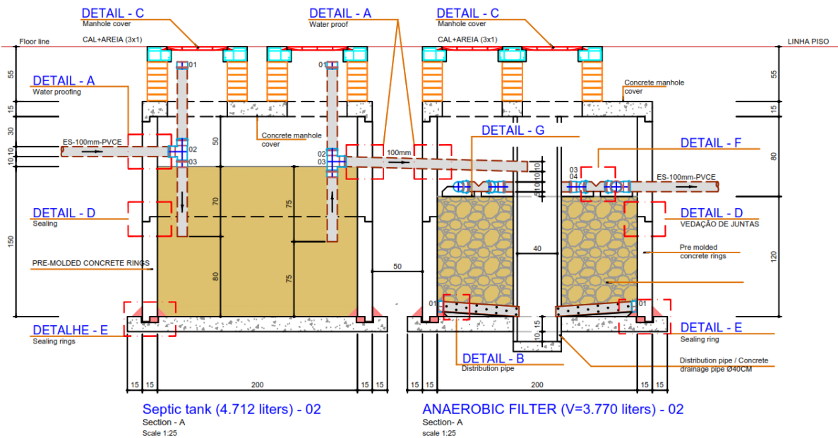
Figure 7: Septic tank proposed in the ISWMC
